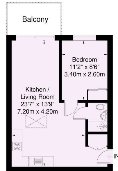
3 Bayldon House Approximate Gross Internal Area = 39.2 sq m / 421 sq ft
